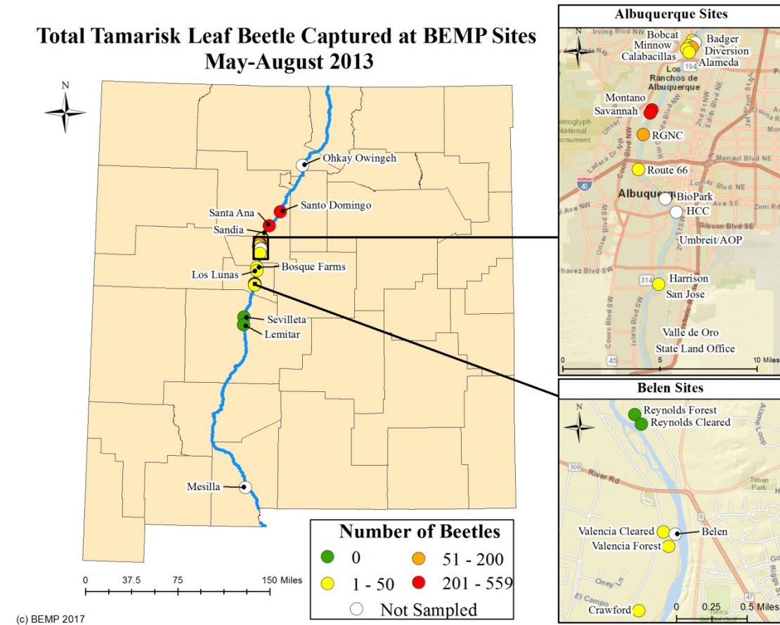
Figure 1. Total TLB captured at BEMP sites from 2013.
