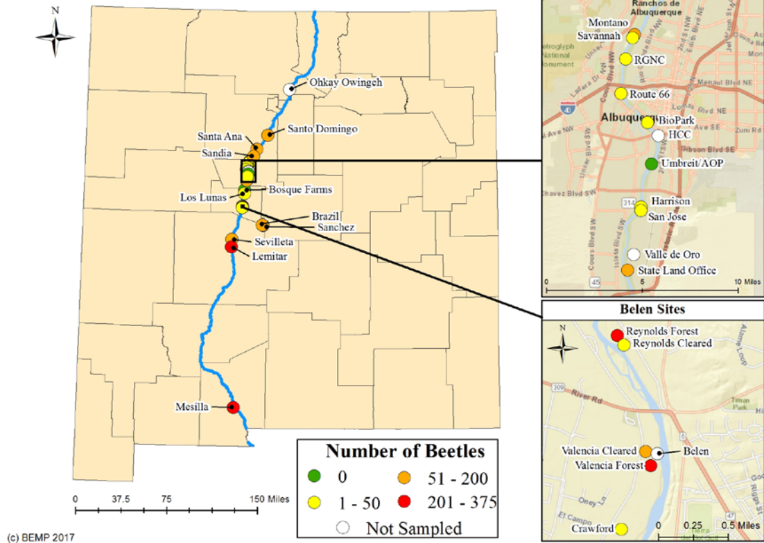
Figure 5. Total TLB captured at BEMP sites from 2017.
