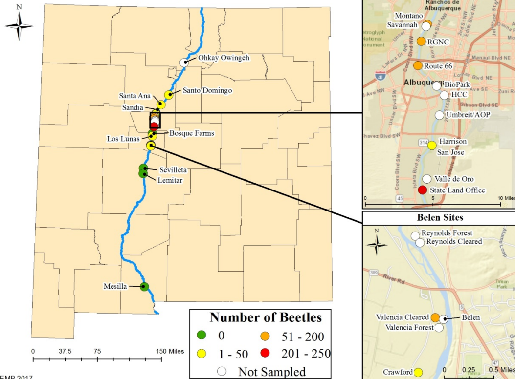
(c) BEMP 2017 Figure 3. Total TLB captured at BEMP sites from 2015.
